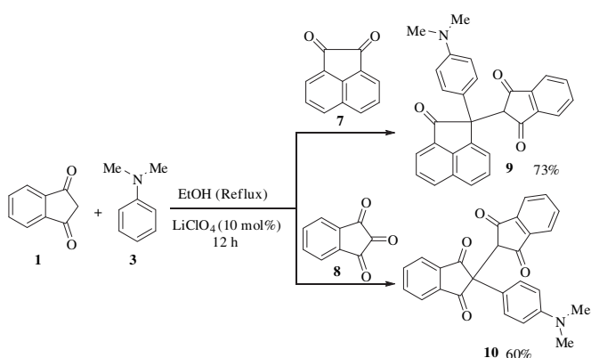
Scheme 3. Examining acenaphthylene-1,2-dione and ninhydrin instead of isatin.
